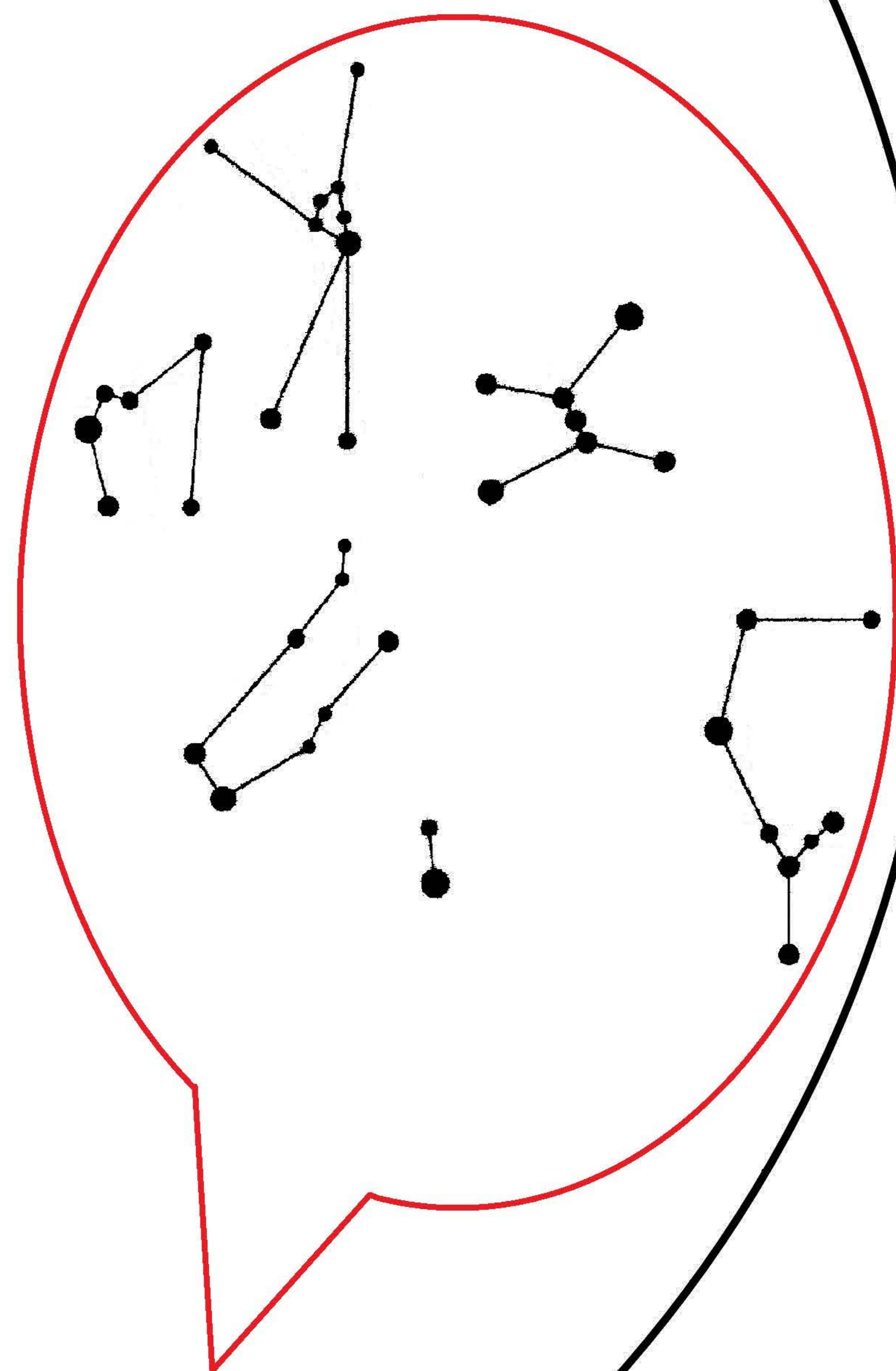
Winter-Sternbilder
